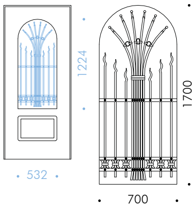
Grata LIBERTY-C 70x170 rA
